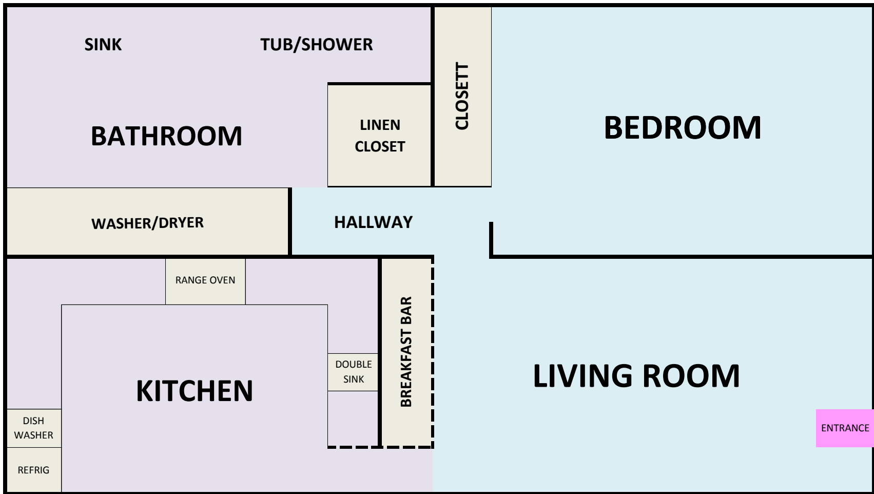
CHARLESTON PLANTATION APARTMENT HOMES 1 BEDROOM - 1 BATH FLOORPLAN
